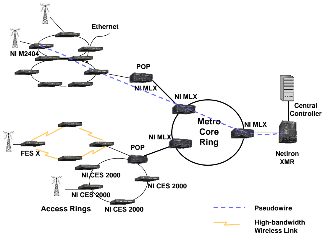
Figure 5 - Example Architecture for Wireless Backhaul using Foundry Routers and Switches
