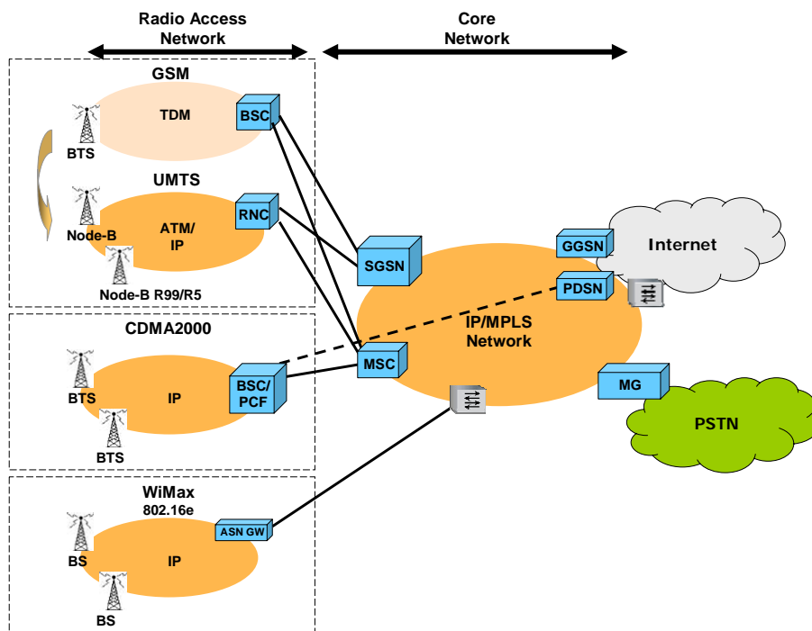
Figure 2 - Reference Architecture for Wireless Carrier Network
