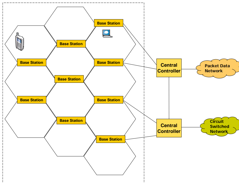
Figure 3 - RAN Architecture
